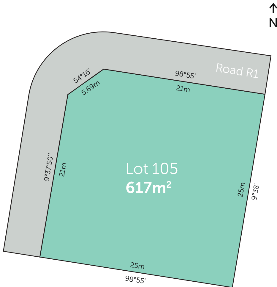
Stage 3 Lot plan
